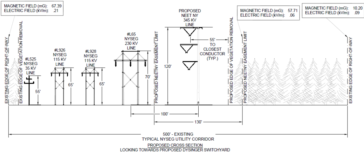
Figure 23 - PROPOSED CROSS SECTION 7 EMF RESULTS
