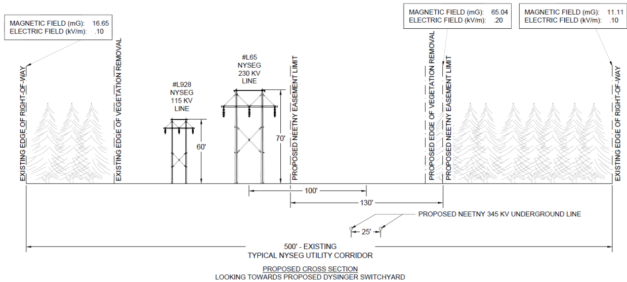
Figure 27 - PROPOSED CROSS SECTION 11 EMF RESULTS
