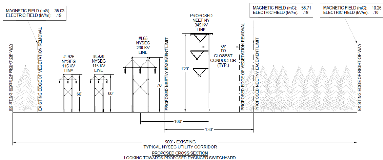
Figure 24 - PROPOSED CROSS SECTION 8 EMF RESULTS
