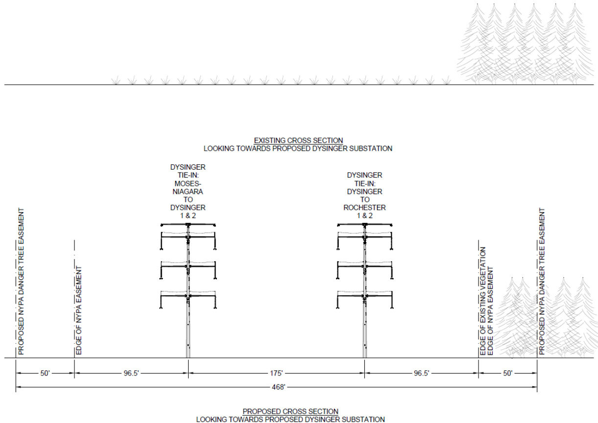
Figure 14 - EXISTING & PROPOSED CROSS SECTION 9
