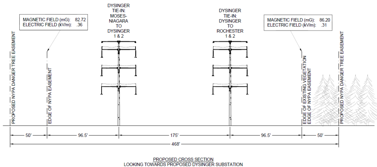
Figure 25 - PROPOSED CROSS SECTION 9 EMF RESULTS
