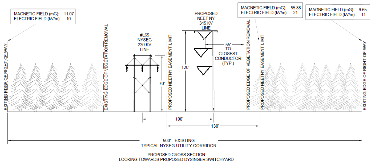
Figure 19 - PROPOSED CROSS SECTION 3 EMF RESULTS
