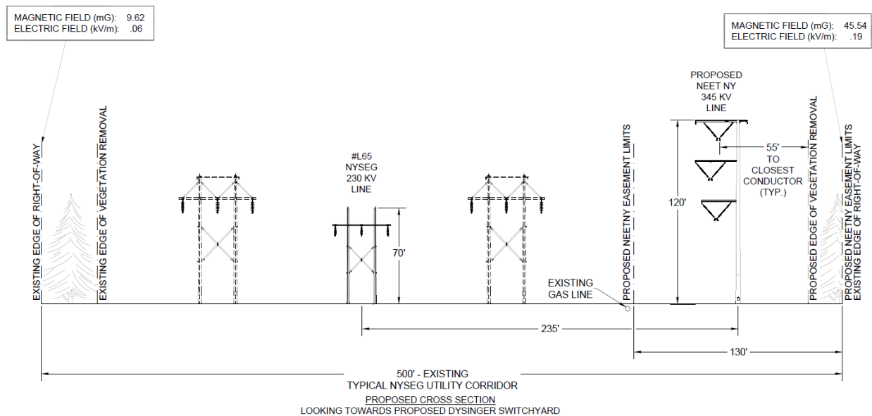
Figure 18 - PROPOSED CROSS SECTION 2 EMF RESULTS
