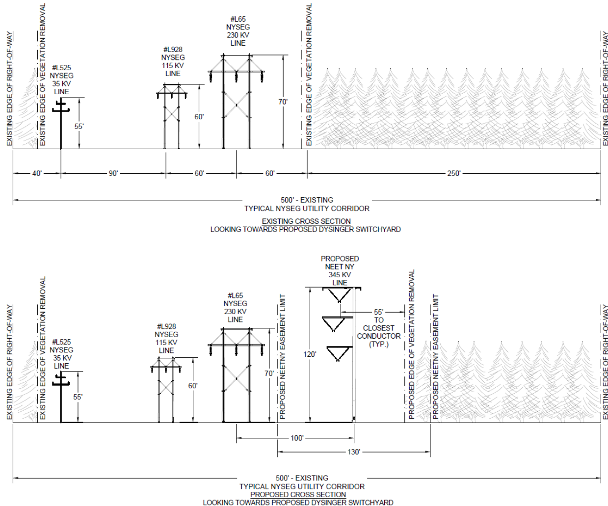
Figure 11 - EXISTING & PROPOSED CROSS SECTION 6
