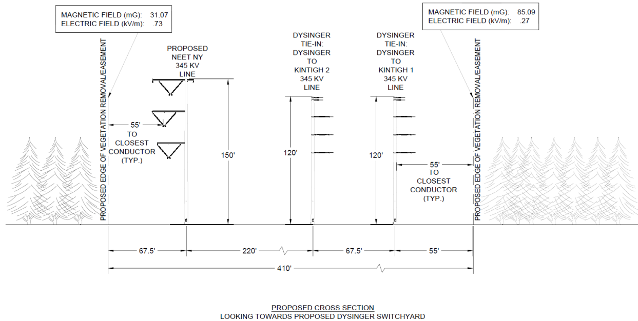
Figure 17 - PROPOSED CROSS SECTION 1 EMF RESULTS
