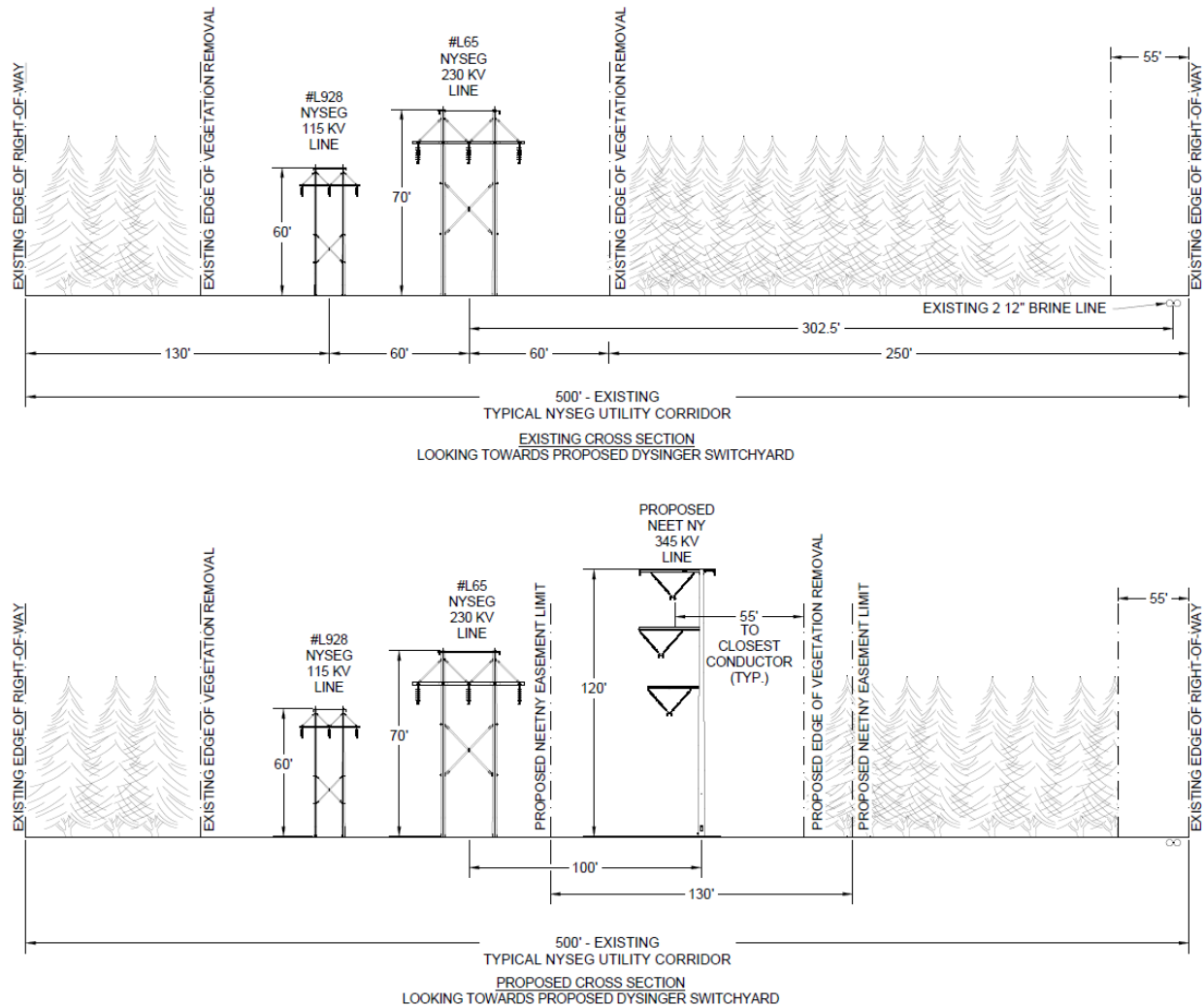
Figure 9 - EXISTING & PROPOSED CROSS SECTION 4
