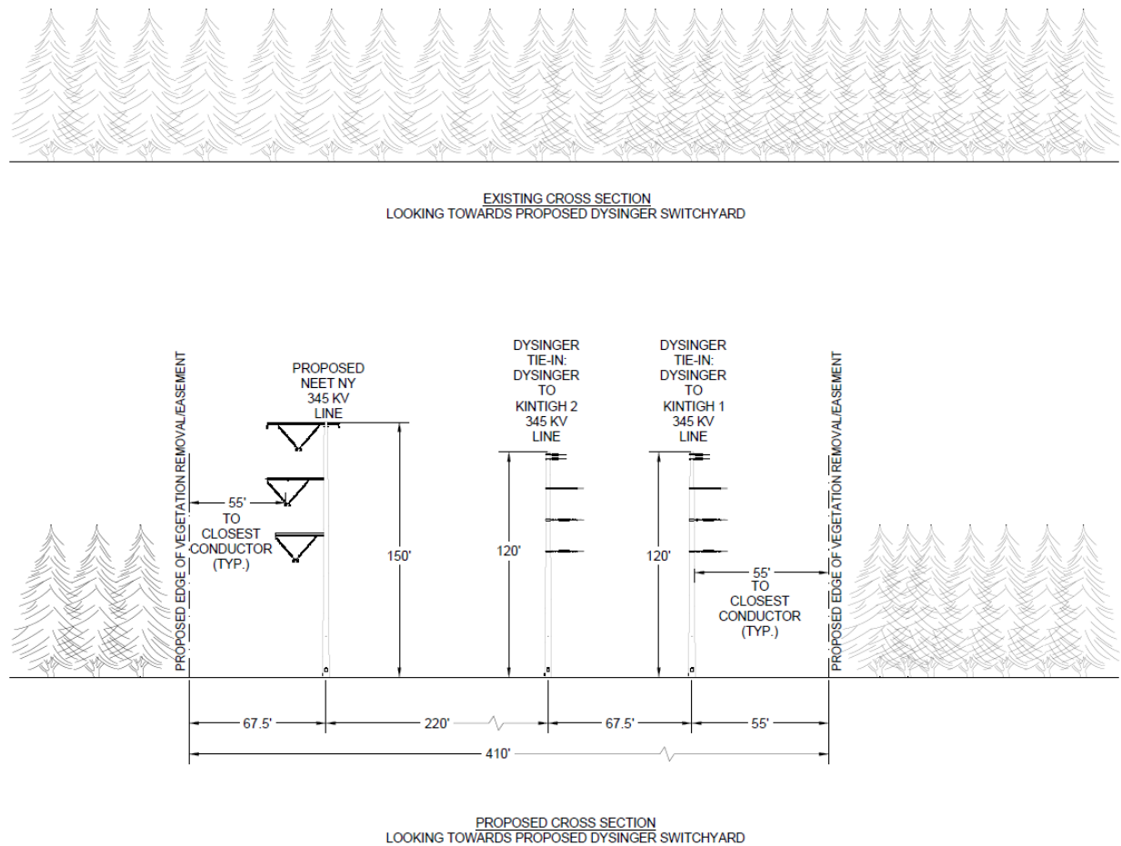
Figure 6 - EXISTING & PROPOSED CROSS SECTION 1
