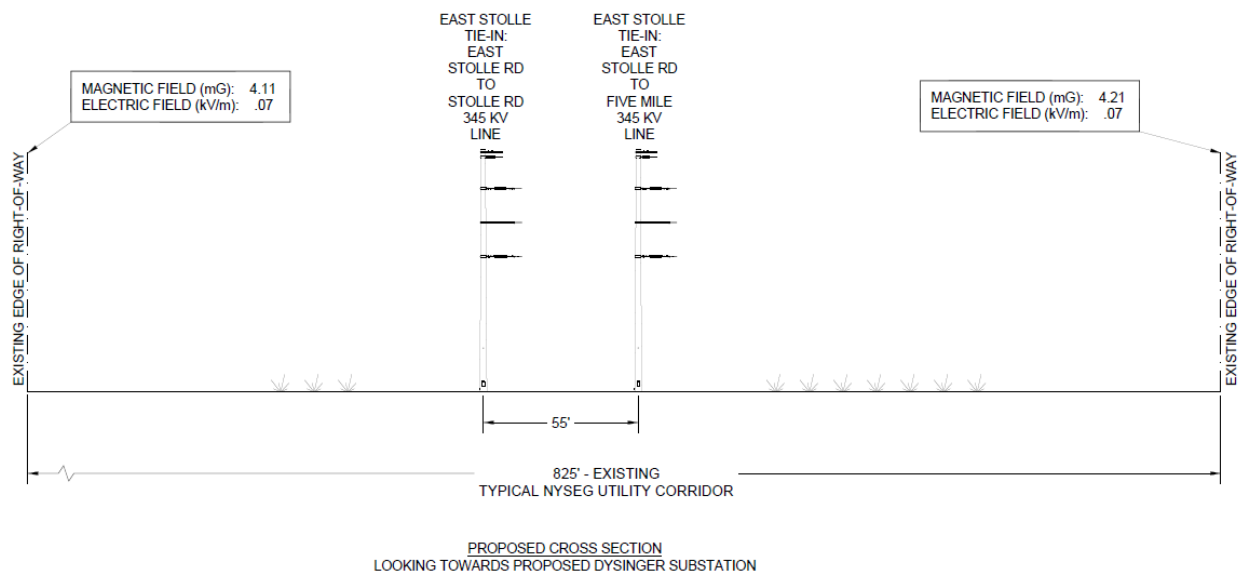
Figure 26 - PROPOSED CROSS SECTION 10 EMF RESULTS
