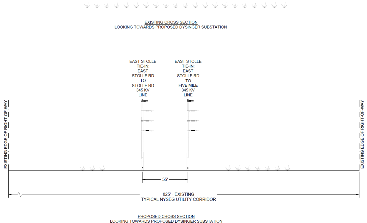
Figure 15 - EXISTING & PROPOSED CROSS SECTION 10
