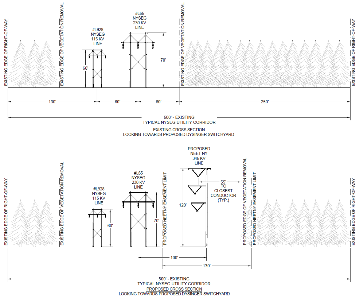
Figure 10 - EXISTING & PROPOSED CROSS SECTION 5
