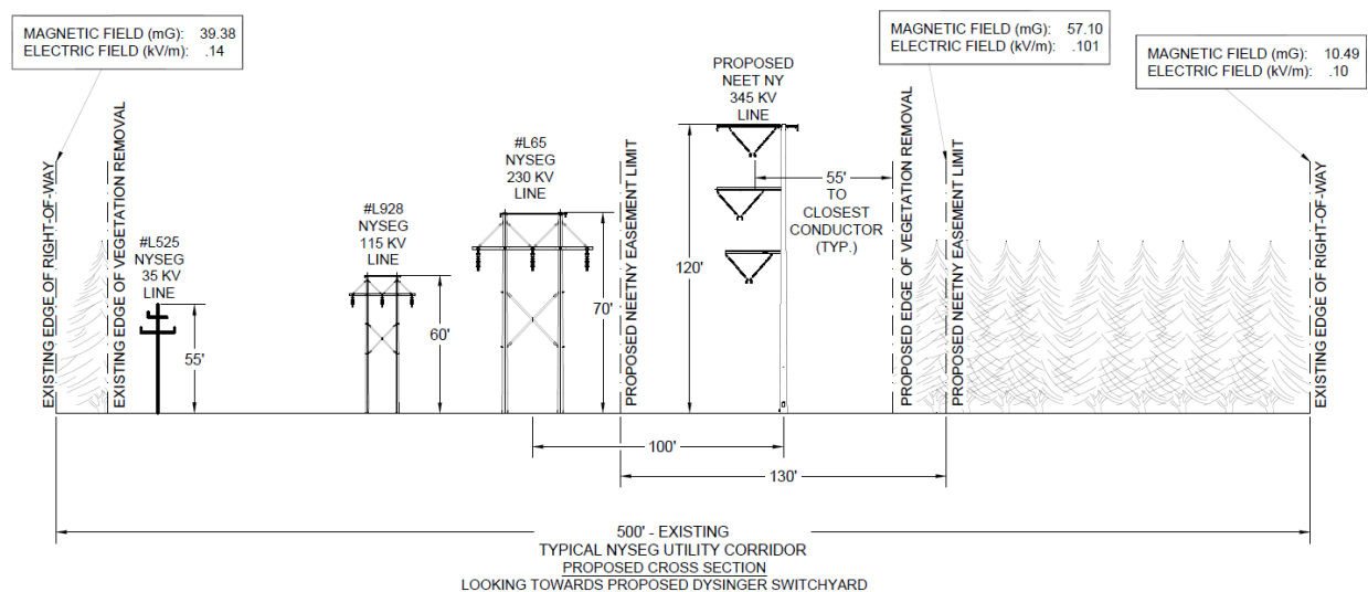
Figure 22 - PROPOSED CROSS SECTION 6 EMF RESULTS
